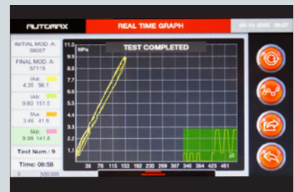
Elastic Modulus test results
